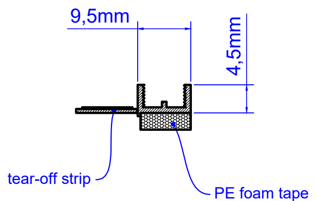
Technical drawing
