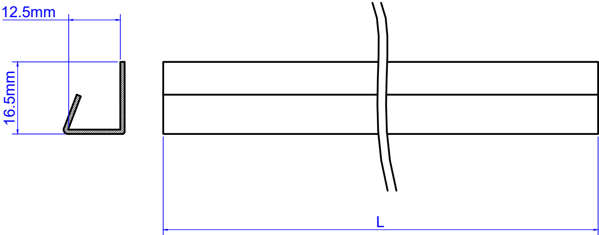
Technical drawing
