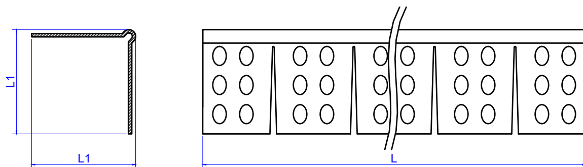
Technical drawing
